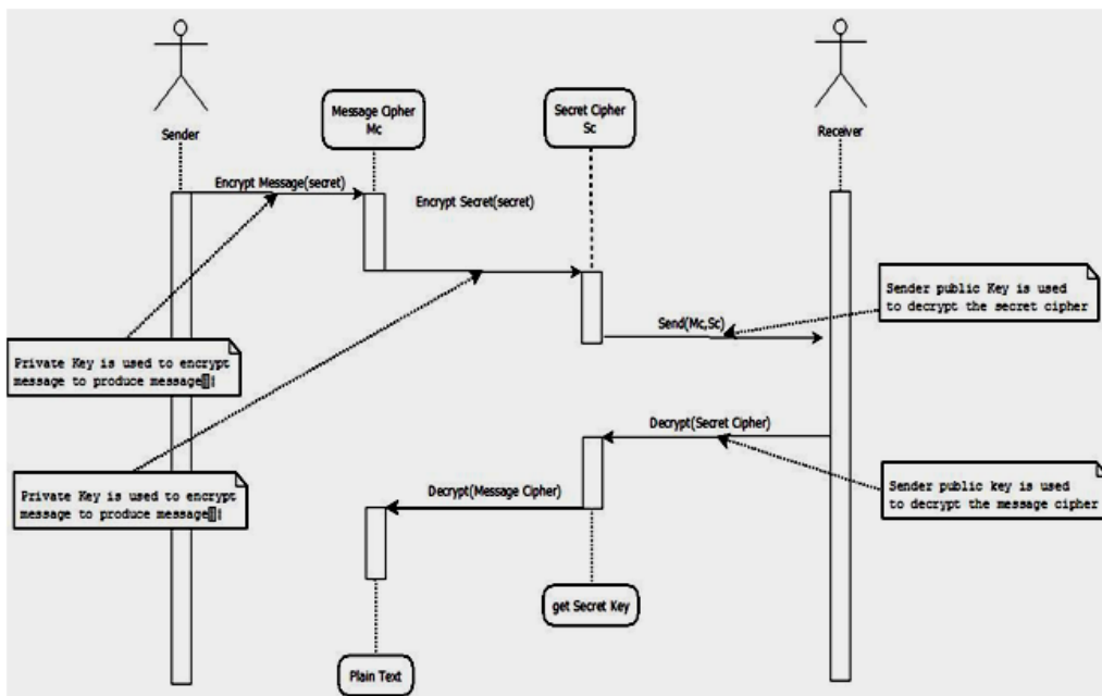
Sequence Diagram of the system
